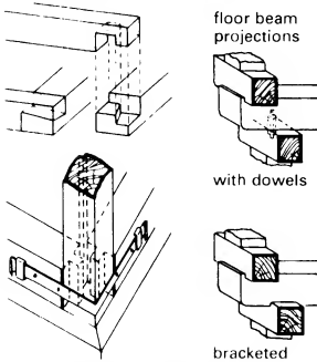
6 Corner connections for framework sills
